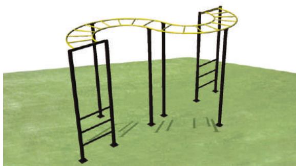
'S' HORIZONTAL LADDER FE36 - H:7ft
